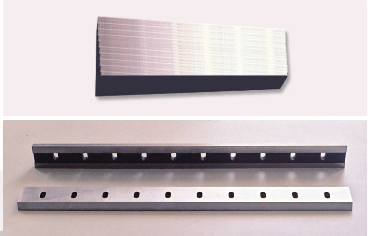
Pictures clockwise from left: 1. Rotary and stationary blades suitable for NGR recycling machine 2. Segments for Pallman pulverizer 3. Polythene cutting blades.
