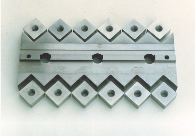
Pictures clockwise from left: 1. Rotary and stationary blades suitable for NGR recycling machine 2. Segments for Pallman pulverizer 3. Polythene cutting blades.
